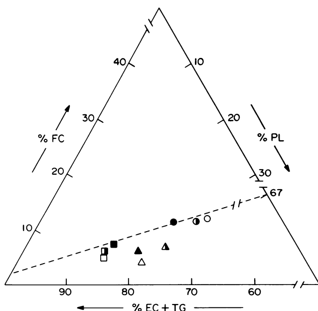
Figure 6. Phase diagram for the lipoprotein average free cholesterol (FC), esterified cholesterol (EC), triglyceride (TG), and phospholipid (PL) moieties of the LDL and VLDL of renal disease and control groups. The dashed line represents the phase boundary above which free cholesterol separates as crystalline phase. Circles, LDL; squares, adsorbed VLDL; triangles, unadsorbed VLDL; open symbols, controls ( n = 10 ); solid symbols, hemodialysis group ( n = 12 ); half-filled symbols, peritoneal dialysis group ( n = 6 ).
