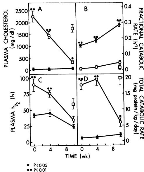
Figure 1. (A) Plasma cholesterol concentrations; (B) fractional catabolic rate of plasma clearance of 125 I-labeled VLDL; (C) half time of elimination of 125 I-labeled VLDL; and (D) total catabolic rate of cholesteryl ester-rich VLDL; in group fed normal diet (●, n = 7), cholesterol-fed group (□, n = 4), and the hypercholesterolemic group returned to a normal diet regimen (○, n = 4). The time axis represents the number of weeks after the hypercholesterolemic animals had been returned to normal laboratory diet. At week 10, a group of continuously cholesterol-fed animals was studied concomitantly with the normal diet fed and previously cholesterol-fed rabbits. Values were measured 0, 4, and 10 wk after the hypercholesterolemic group had been returned to a normal diet regimen and are means ± standard errors. * P < 0.05; ** P < 0.01.
