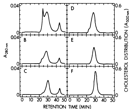
Figure 4. High performance liquid chromatography subfractionation by size of plasma VLDL after reinstatement of a normal chow regimen. Absorbance at 280 nm ( A_{280\text{nm}} ) was recorded for VLDL obtained from rabbit plasma after animals had been returned to a normal laboratory diet regimen at (A) 0, (B) 4, and (C) 10 wk. The distribution of cholesterol within the subfractions is illustrated in D, E, and F.
